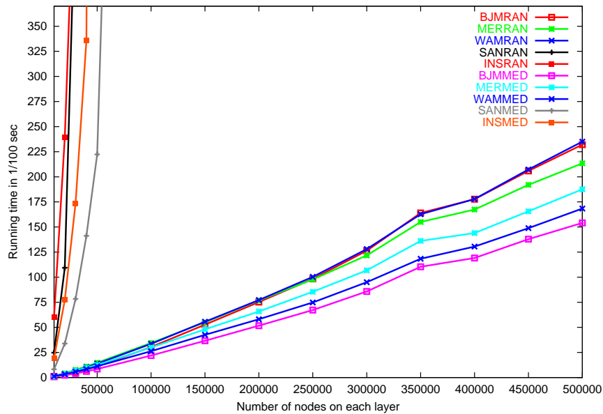
Figure 7: Running time for large sparse graphs
