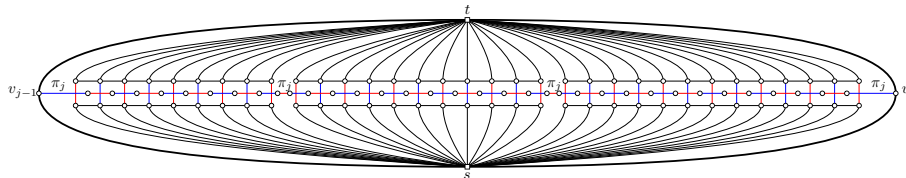
Figure 7: Illustration of a wedge in the construction for the 1-SEFE problem.
