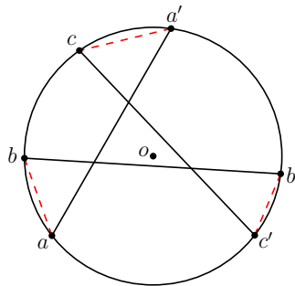
Figure 6: Proof of case (i) in Theorem 1.
