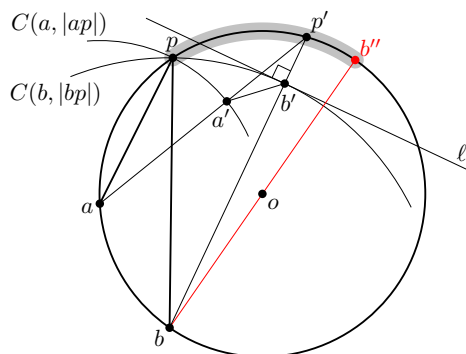
Figure 4: Proof of Lemma 4.
