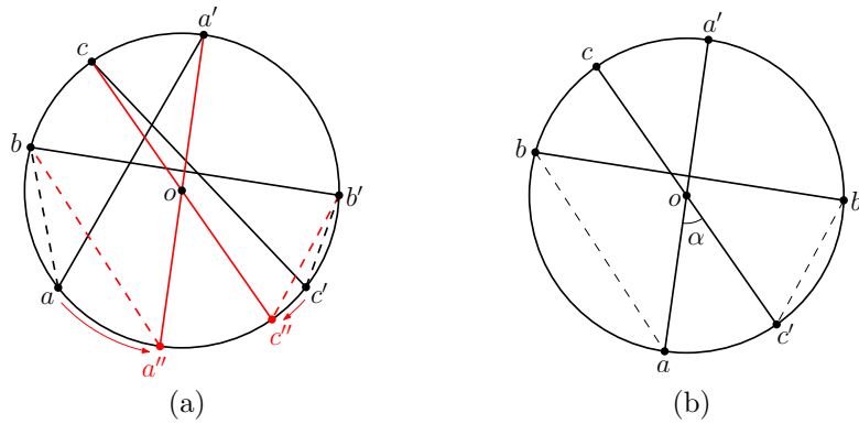
Figure 7: Proof of case (ii) in Theorem 1.
