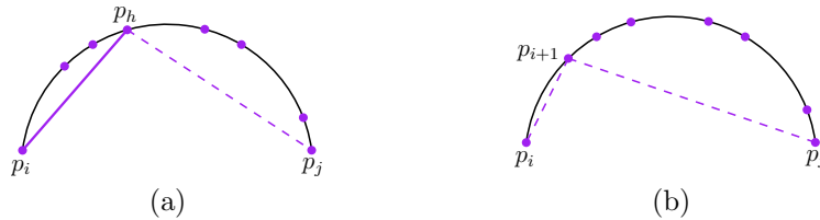
Figure 1: Solving subproblem (i, j) : (a) p_i is connected to a purple point p_h , and (b) p_i is not connected to any purple point.
