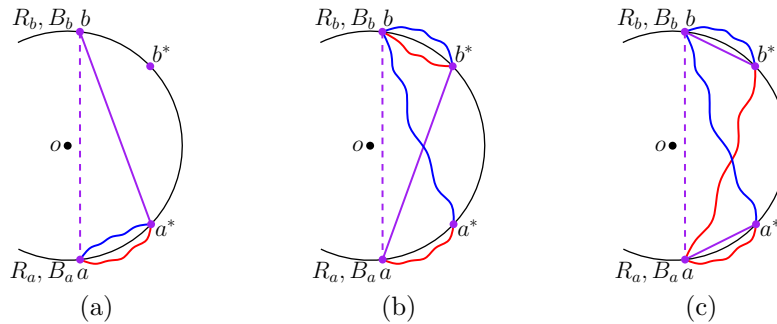
Figure 2: Proof of Lemma 2: (a) a^* \in R_a and a^* \in B_a . (b) a^* \in R_a and a^* \in B_b . (c) a^* \in B_b and b^* \in R_a .
