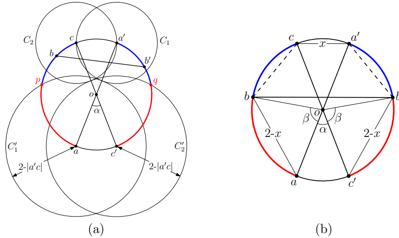
Figure 8: Proof of case (ii) in Theorem 1.
